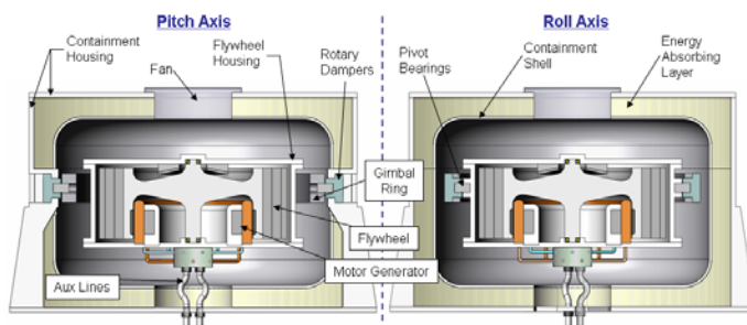
Figure 9: Containment structure for arbor flywheel
